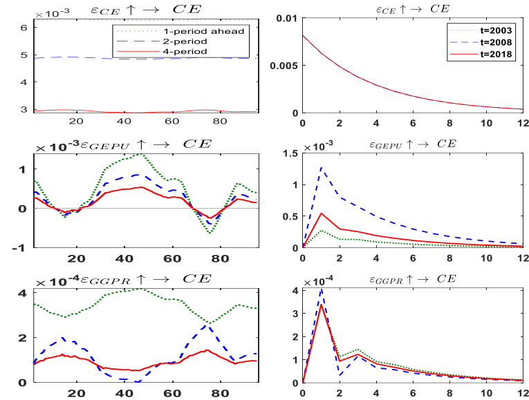
Figure 13: Global data equal interval and point-in-time impulse response
